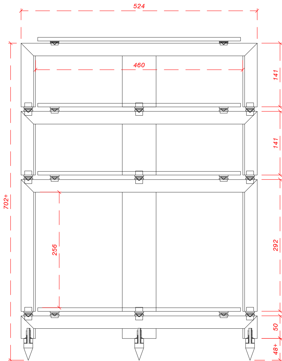
2x Standard Height & 1x Double Height Levels 1x Base Level
