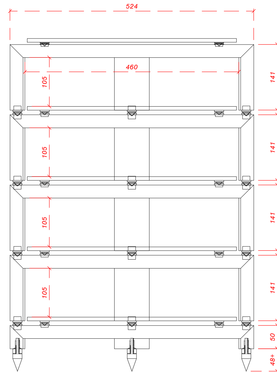
4x Standard Height Levels 1x Base Level
